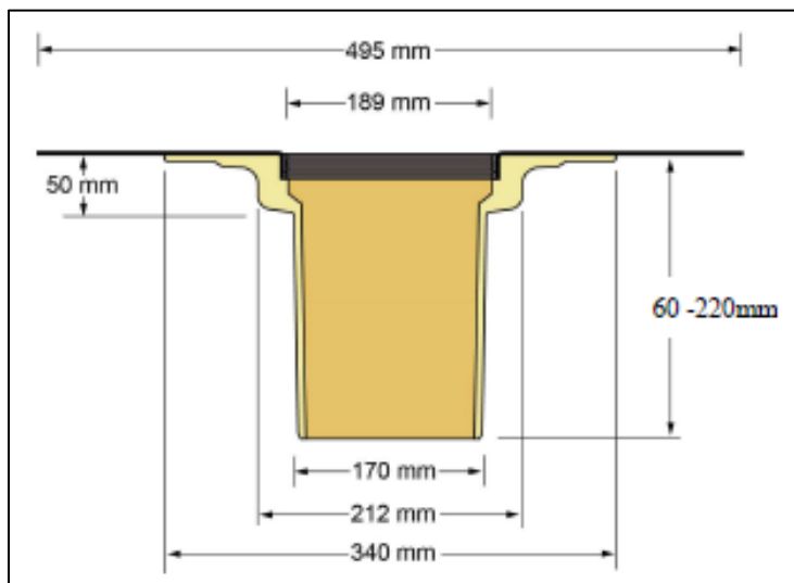
Bitumen Vertical Outlet Extension Unit
