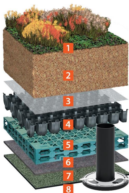
Indicative sedum blue roof system
