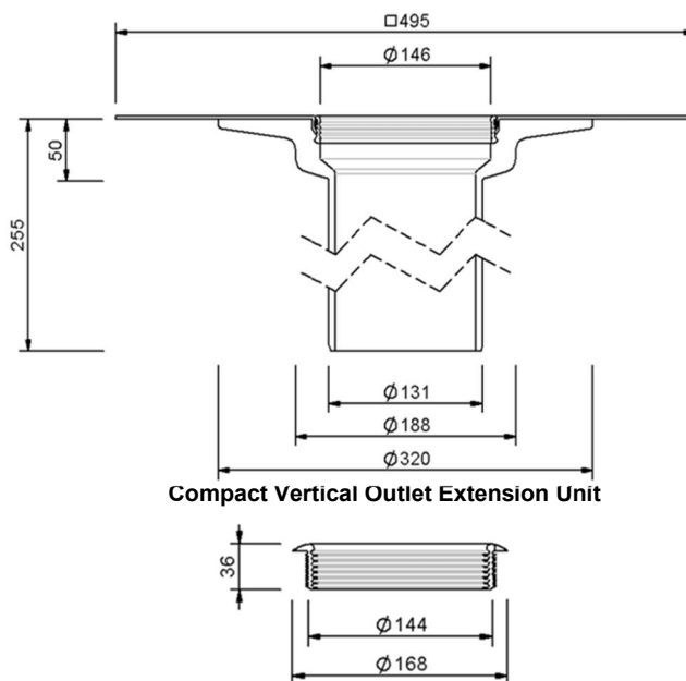
Webbed Insertion Flange
